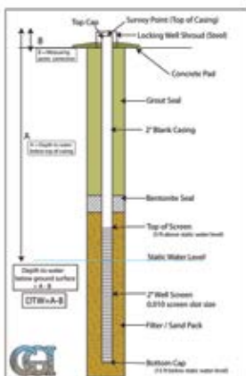
Figure 1. Ground water monitoring well completion schematic (modified from NWED Groundwater Discharge Permit Monitoring Well Construction and Abandonment Guidelines, 07/06)
